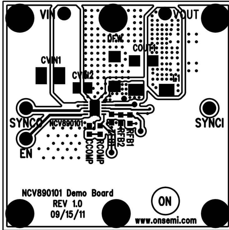
Figure 16. Top View
