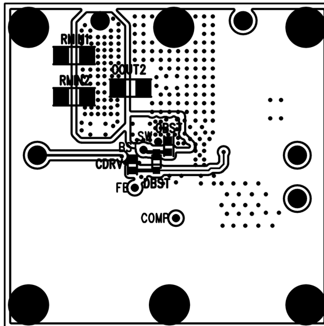
Figure 17. Bottom View
