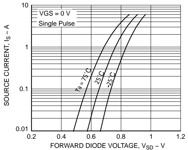
Figure 7. I_S - V_{SD}
