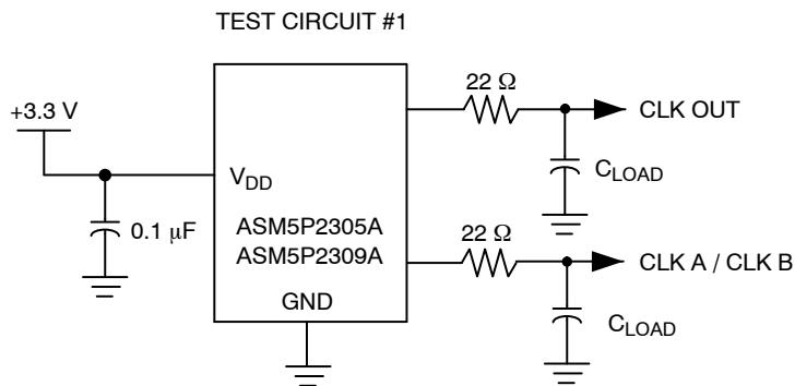
Figure 3. Test Circuit
