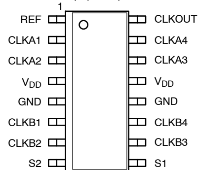
ASM5P2309A (Top View)
