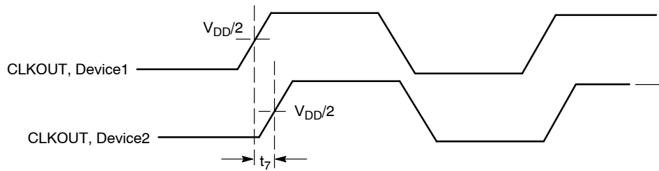
Figure 8. Device-Device Skew
