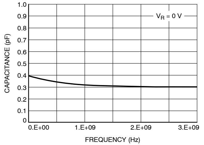
Figure 6. Typical Capacitance over Frequency ESD7410N2T5G
