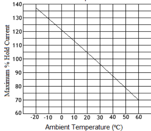
Ambient Compensation Chart
