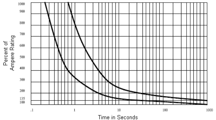
Part number: MRCBP4-PM Time Current Curves
