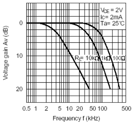
Fig.11 Frequency Response
