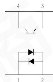
1. Anode, Cathode 3. Emitter 2. Cathode, Anode 4. Collector
