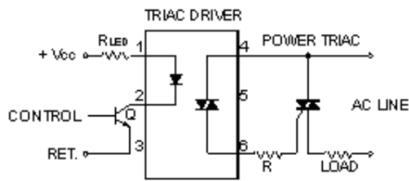
Basic Driver Circuit
