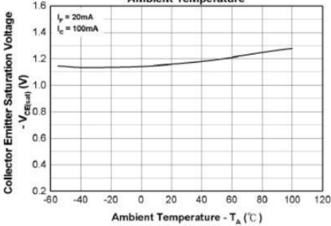
Figure 3. Collector Emitter Saturation Voltage vs. Ambient Temperature
