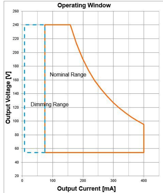
Operating Window ETI DALI 35/220-240/400 D LT2 L
