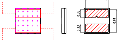
Component Location on Pad
