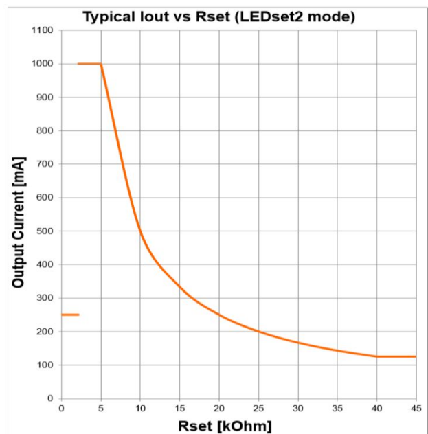
OTI DALI 150/220-240/1A0 D NFC IND L Typical Iout vs Rset (LEDset2 mode)
