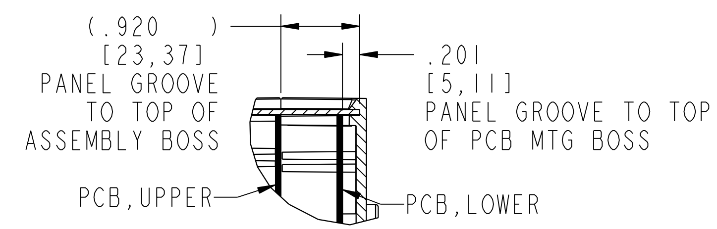
DETAIL D PCB MOUNTING OPTIONS SCALE 0.900
