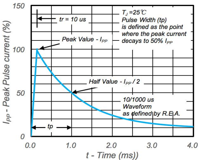
Fig.3 Pulse Waveform
