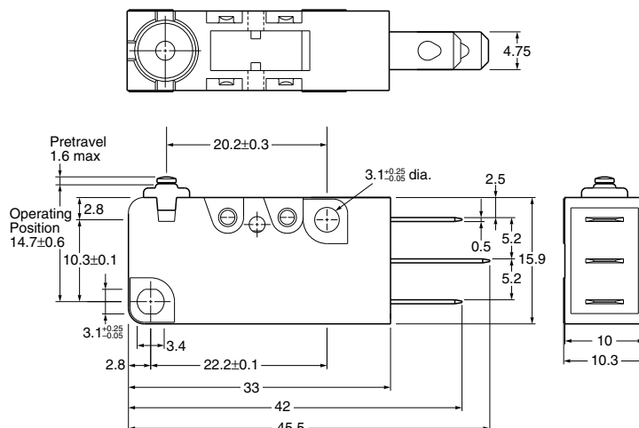
External dimensions
