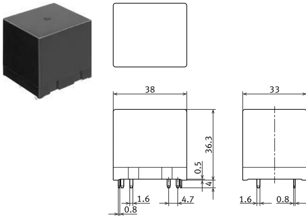
External dimensions
