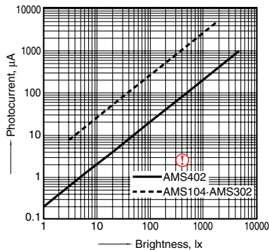
4. Photocurrent vs. brightness characteristics Light source: Fluorescent lamp Reverse voltage: 3V (AMS402), 5V (AMS104, AMS302) Ambient temperature: 25°C 77°F
