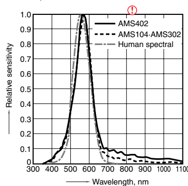
2. Relative sensitivity vs. wavelength characteristics Reverse voltage: 3V (AMS402), 5V (AMS104, AMS302) Ambient temperature: 25°C 77°F
