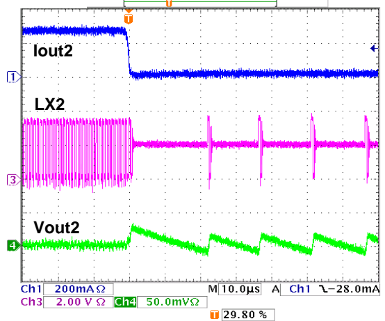
DC-DC2 Iout2 = 250 mA to 10 mA , Δ t = 1 μsec
