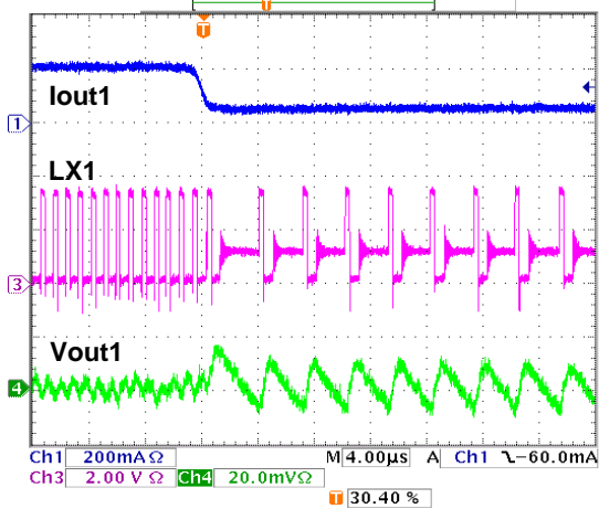
DC-DC1 Iout1 = 200 mA to 50 mA , Δ t = 1 μsec
