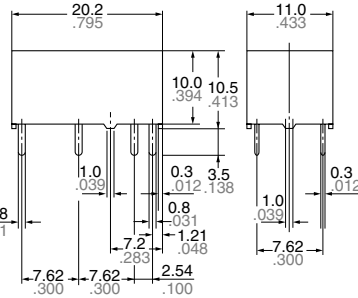
2 coil latching
