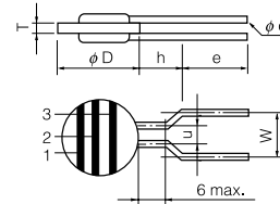
Crimped Lead Type Z Type
