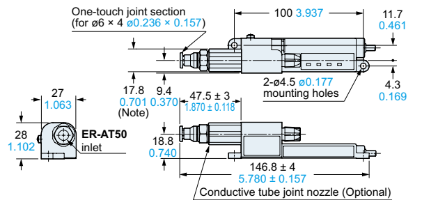
Mounting drawing with conductive tube joint nozzle (ER-VAJT-64, Optional)
