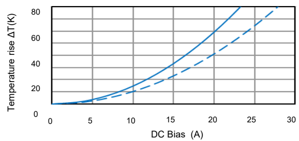
[ ETQP6M2R5YSC ]
