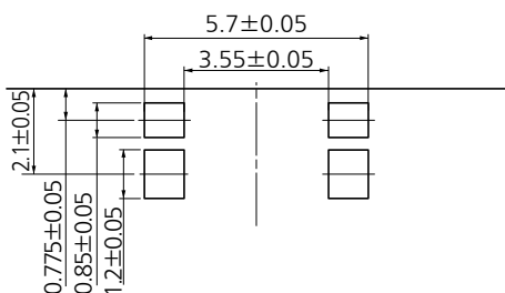
Recommended Solder Mask A
