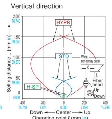
FD-60 Reflective type
