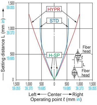
FT-A11V Thru-beam type
