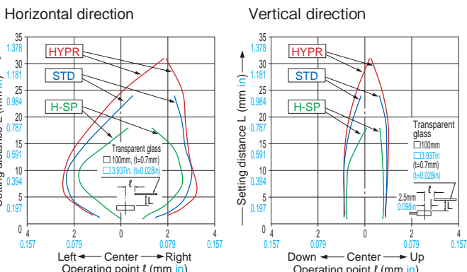
FD-L30A Reflective type
