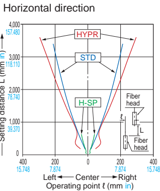
FT-Z30HW Thru-beam type
