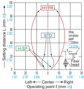
FD-H18-L31 Reflective type
