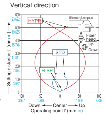
FD-41W Reflective type
