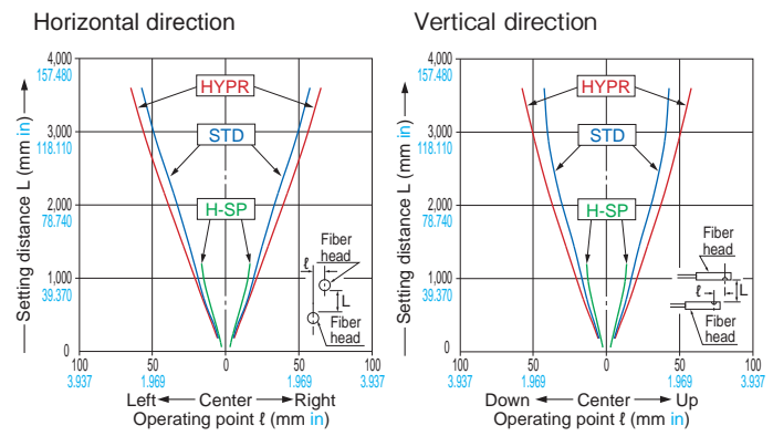
FT-R40 Thru-beam type
