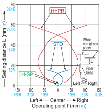
FD-S32 Reflective type
