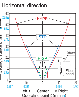
FR-KZ22E Retroreflective type
