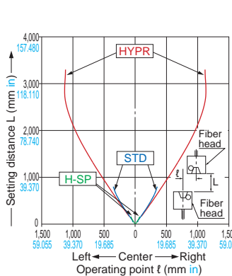
FT-Z40HBW Thru-beam type
