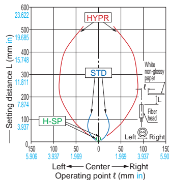
FD-S32W Reflective type
