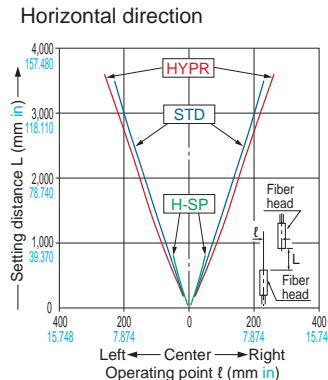
FT-Z30W Thru-beam type
