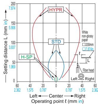
FD-S31 Reflective type
