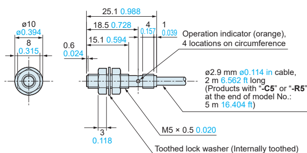
GX-305M-□ Sensor
