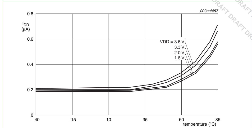
Fig 10. Deep power-down mode: Typical supply current I_{DD} versus temperature for different supply voltages V_{DD}
