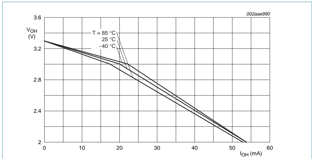
Fig 11. High-drive output: Typical HIGH-level output voltage V_{OH} versus HIGH-level output current I_{OH} .
