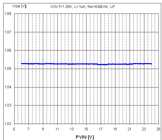
Frequency = 630 kHz
