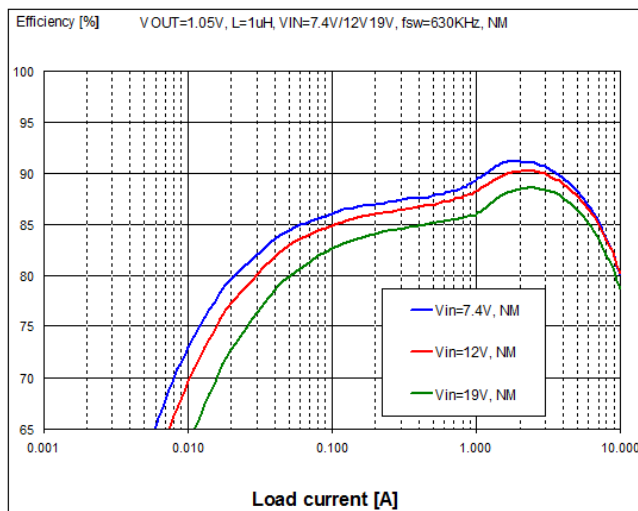
V_{OUT} = 1.05\text{ V} , L_o = 1\text{ }\mu\text{H}
