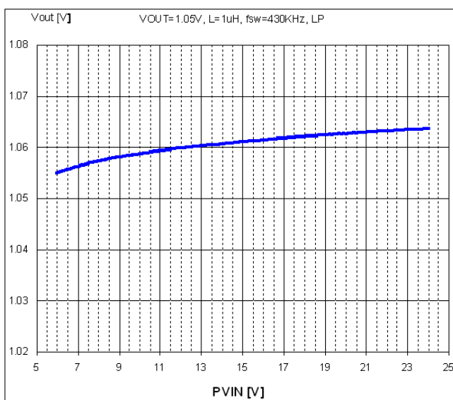
Frequency = 430 kHz
