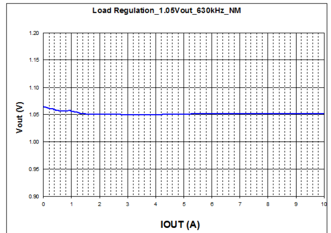
Frequency = 630 kHz
