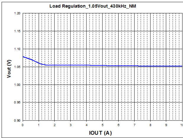
Frequency = 430 kHz
