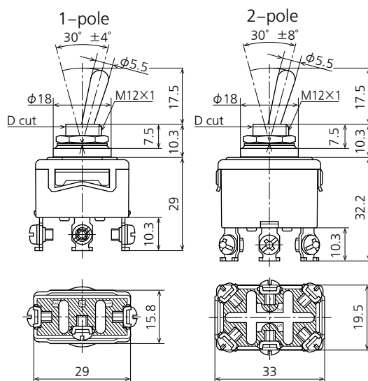
External dimensions
