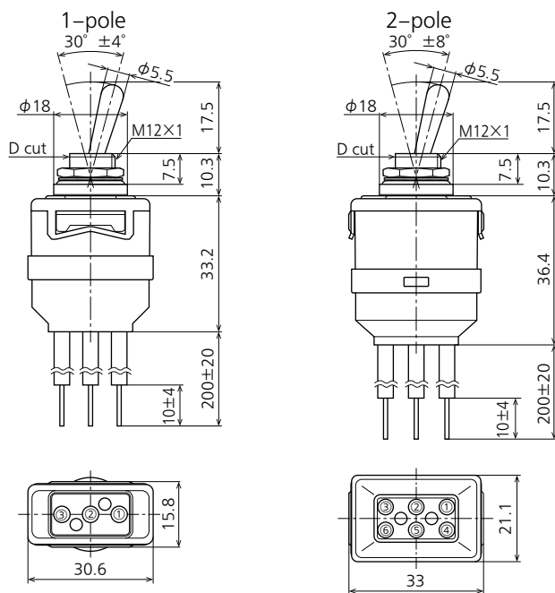
External dimensions
