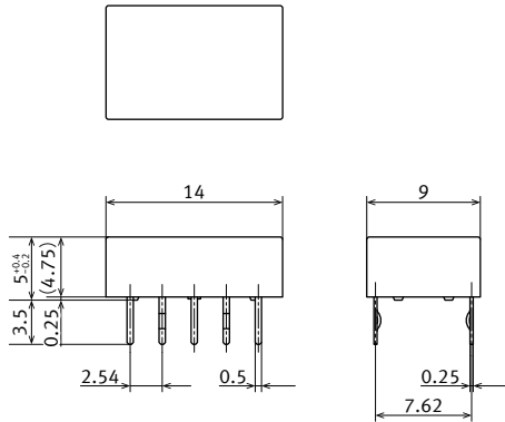
PC board terminal (self-clinching terminal)
