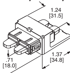
SC Duplex Adapter
