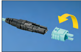
Remove Outer Housing, Flip and Reinstall
