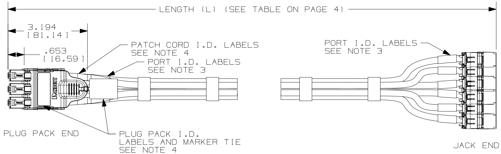
(QPJ***** ) 6-CABLE ASSEMBLY PLUG PACK TO LOOSE JACKS SHOWN
