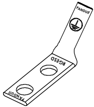
TWO HOLE ESD PORT BENT 45° (QTY. 1)
