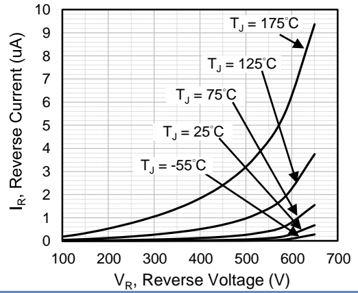
Fig.2 Reverse Characteristics
