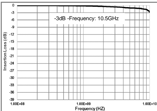
Fig.5 Insertion Loss
