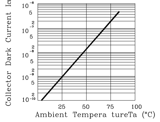
Fig. 2 Collector Dark Current I cb (A) vs. Ambient Temperature
