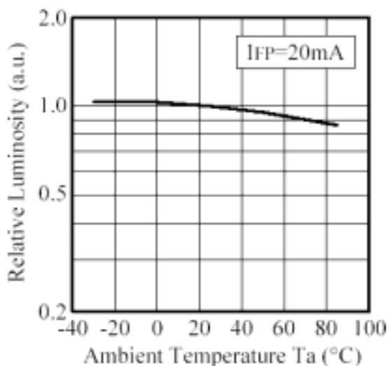
■ Ambient Temperature vs. Relative Luminosity
