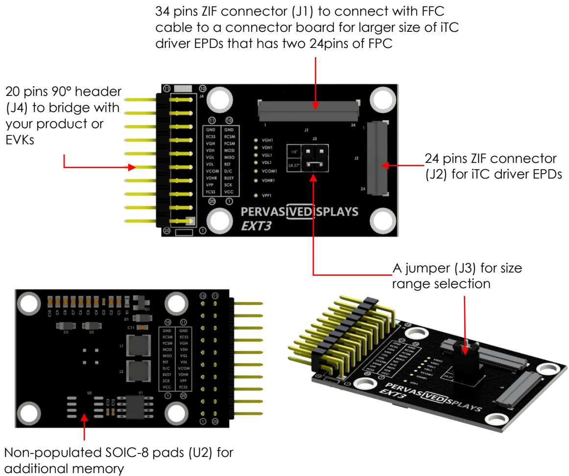
Figure 3 Overview of EXT3 board
