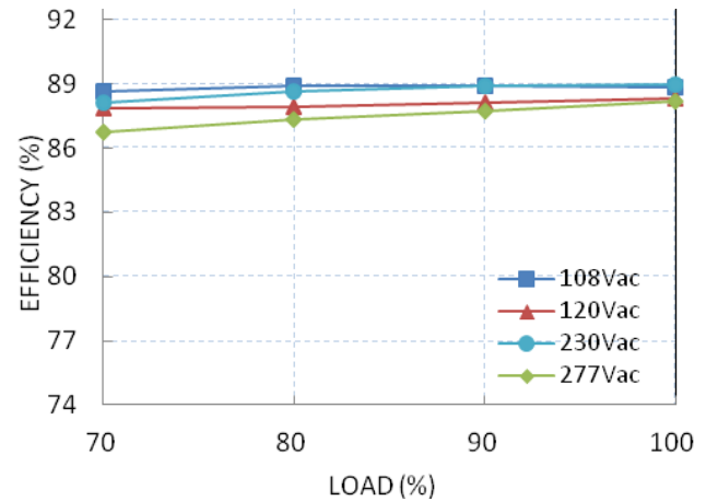
Efficiency vs. Load (PDA041B-700B)
