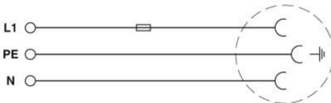
Circuit diagram
