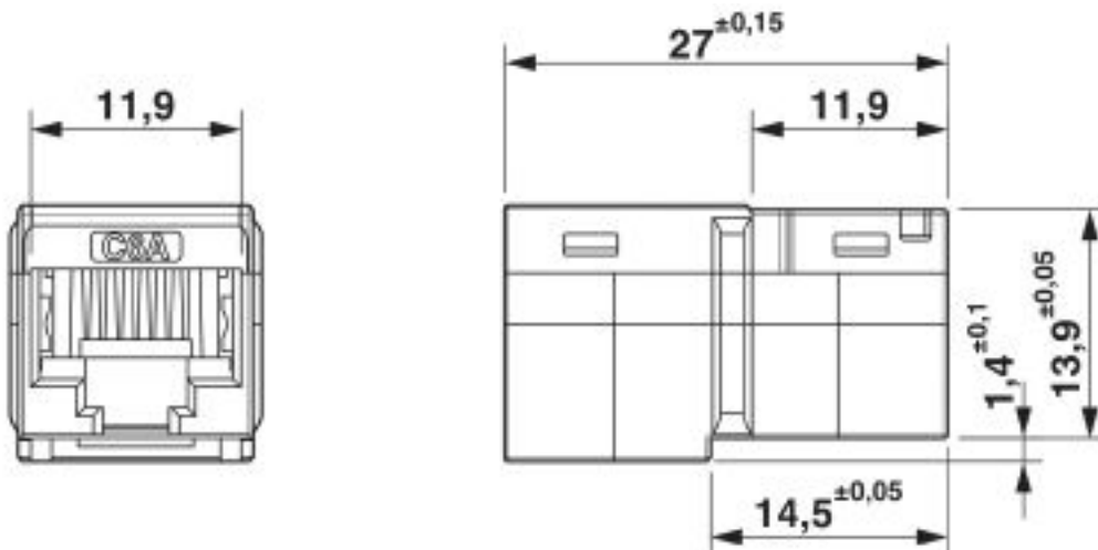
Dimensional drawing
