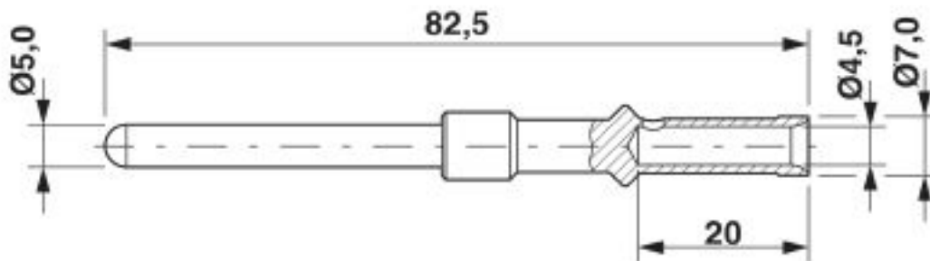
Dimensional drawing
