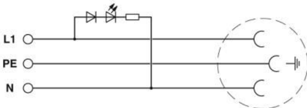
Circuit diagram
