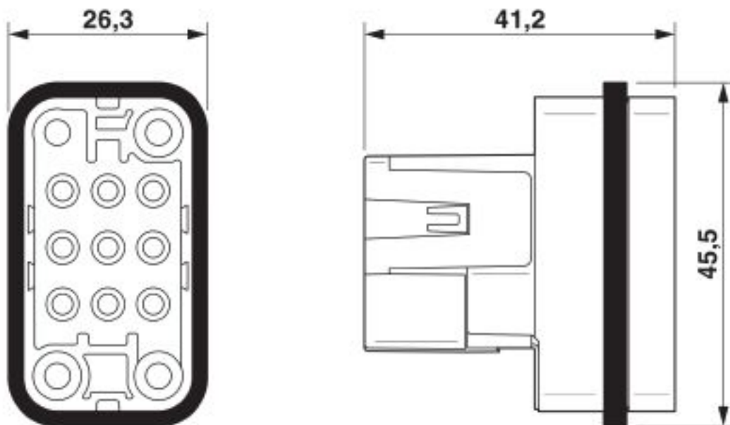
Dimensional drawing
