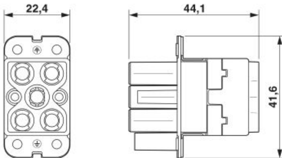
Dimensional drawing
