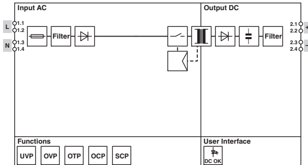
Figure 4 Block diagram
