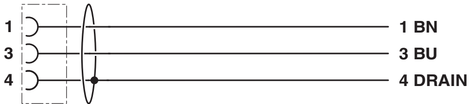
Contact assignment of M8 plugs/sockets
