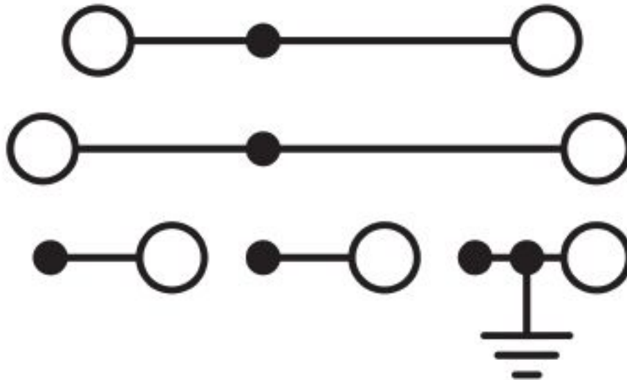
Circuit diagram
