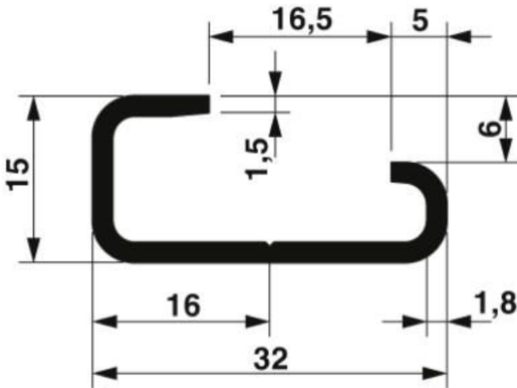
Dimensional drawing
